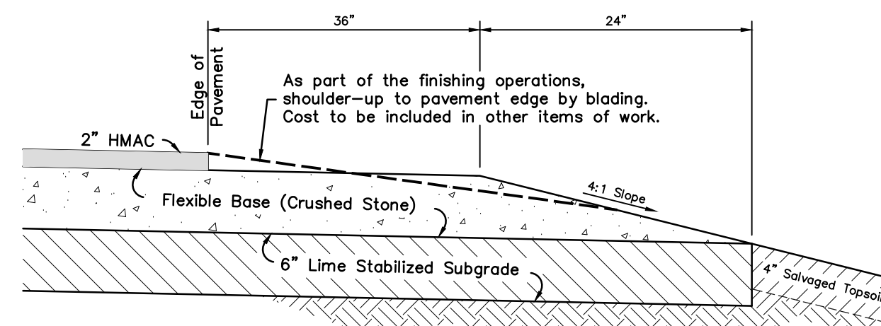
TYPICAL SHOULDER DETAIL
